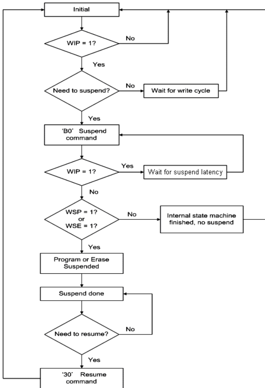
Write Suspend/Resume Flow
