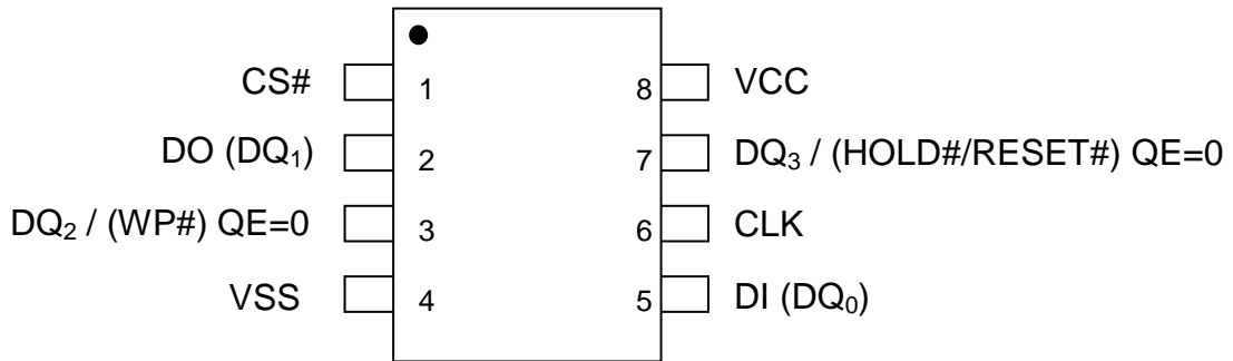
8 – LEAD SOP
