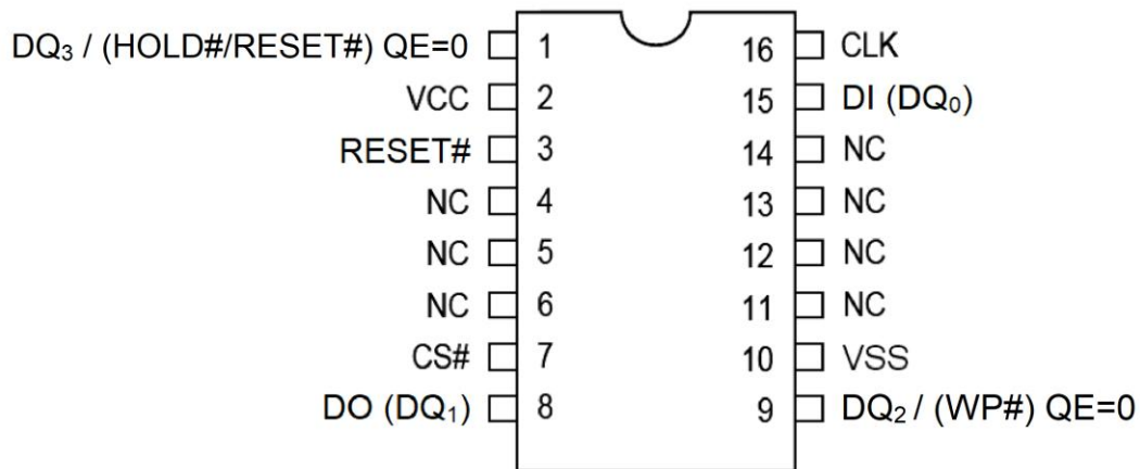
16 – LEAD SOP
