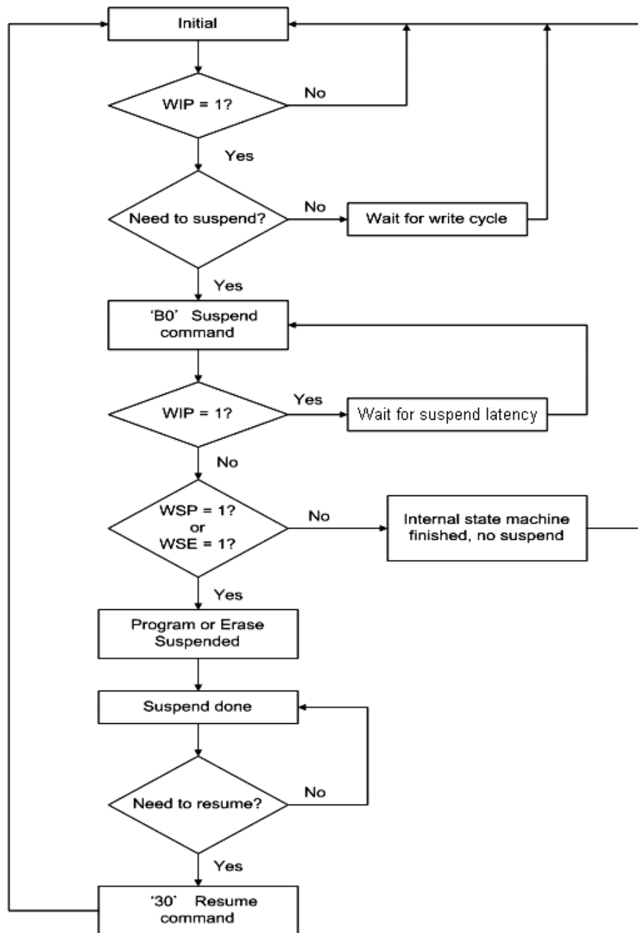
Figure 27. Write Suspend/Resume Flow
