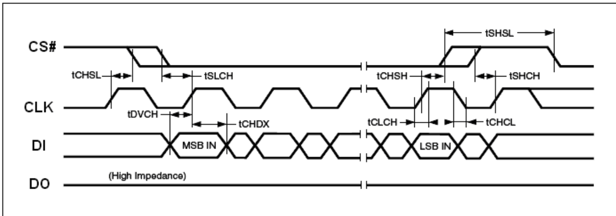
Figure 42. Input Timing
