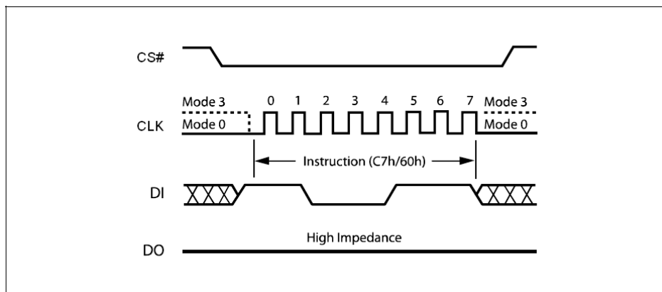
Figure 31. Chip Erase Instruction Sequence Diagram
