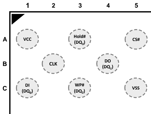
WLCSP (Package Code: SP)
