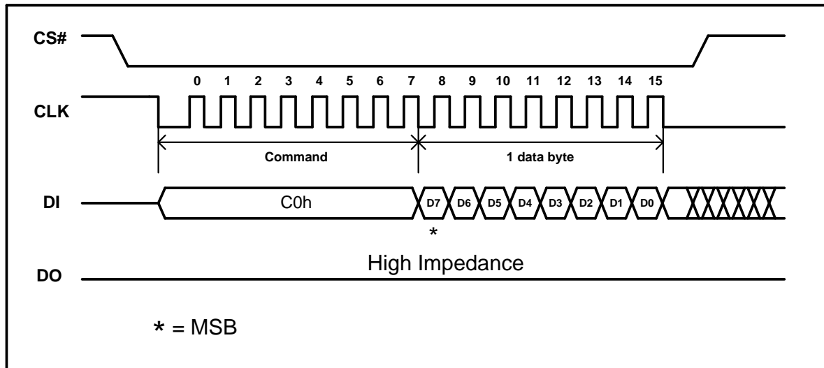
Figure 20. Set Burst Instruction Sequence Diagram
