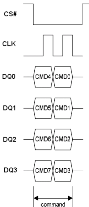
Figure 26.1 Write Suspend/Resume Instruction Sequence in QPI Mode
