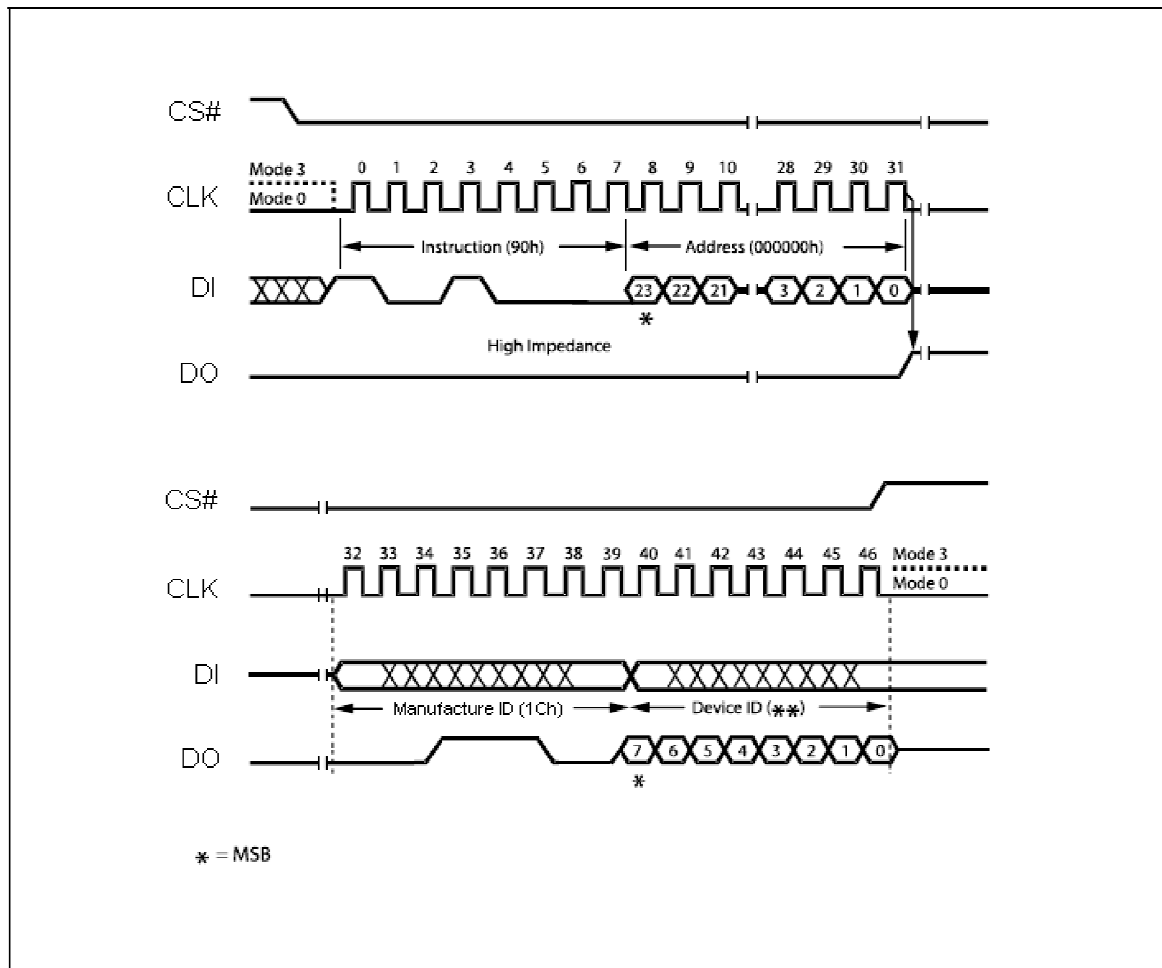
Read Manufacturer / Device ID Diagram
