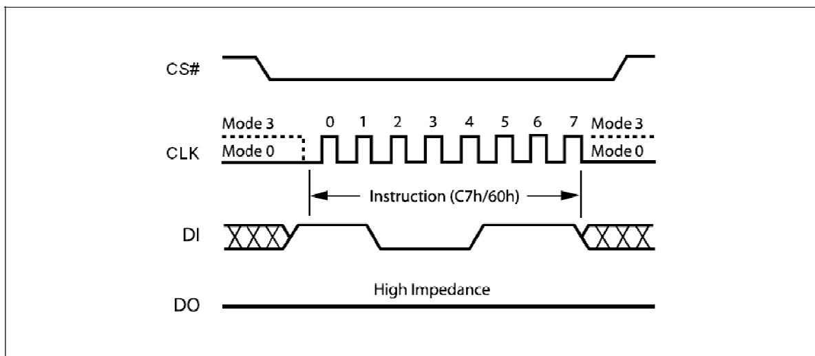
Chip Erase Instruction Sequence Diagram
