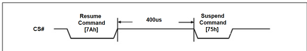
Resume to Suspend Latency
