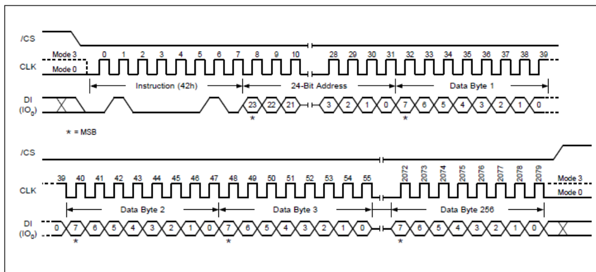
Program OTP array
