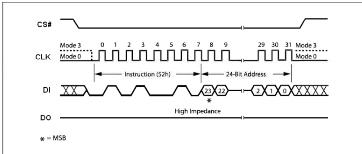
32KB Half Block Erase Instruction Sequence Diagram
