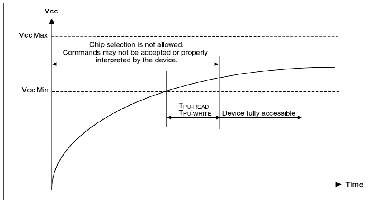
Power-up Timing
