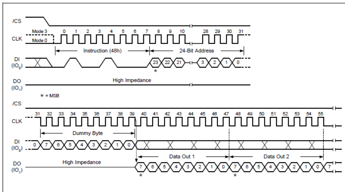
Read OTP array
