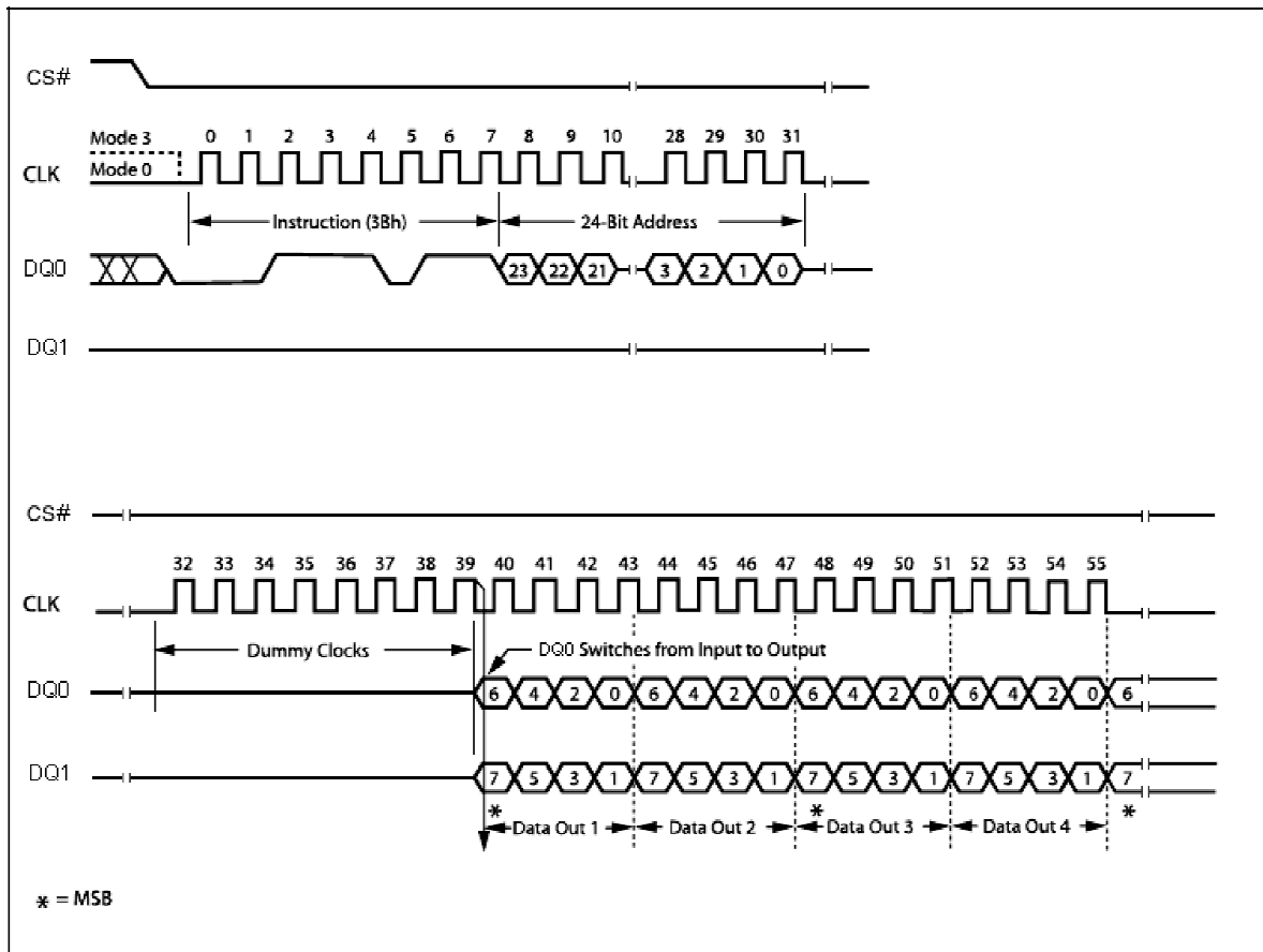
Dual Output Fast Read Instruction Sequence Diagram
