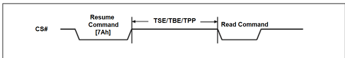
Resume to Read Latency
