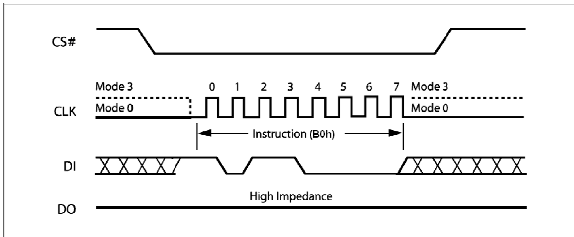
Write Suspend Instruction Sequence Diagram
