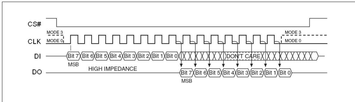
SPI Modes
