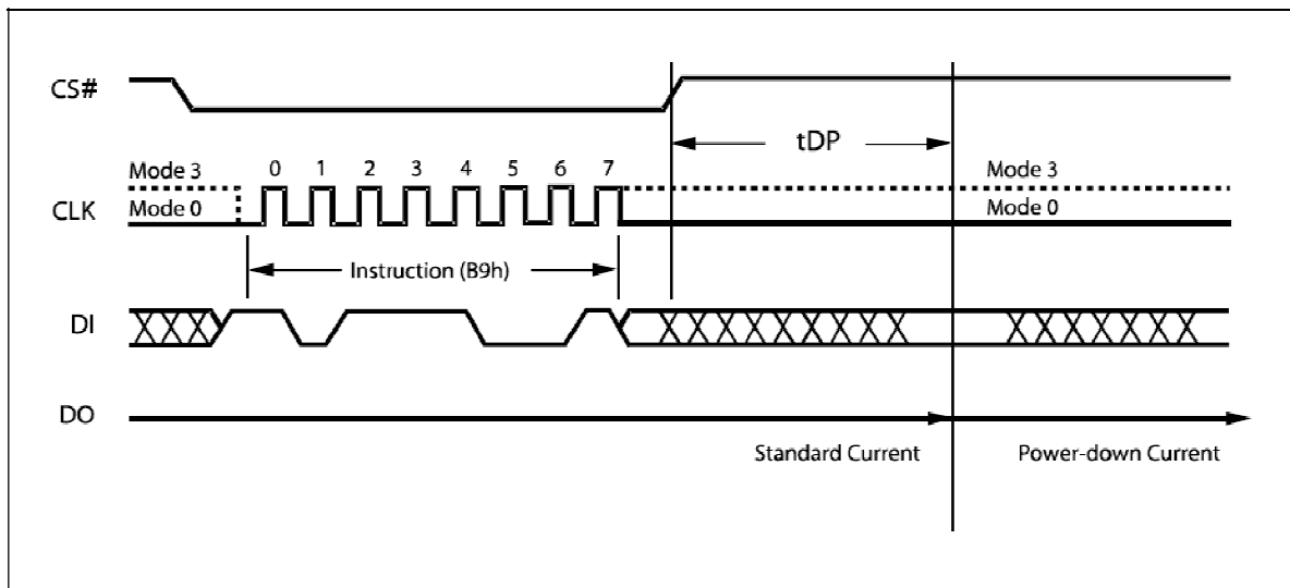
Deep Power-down Instruction Sequence Diagram
