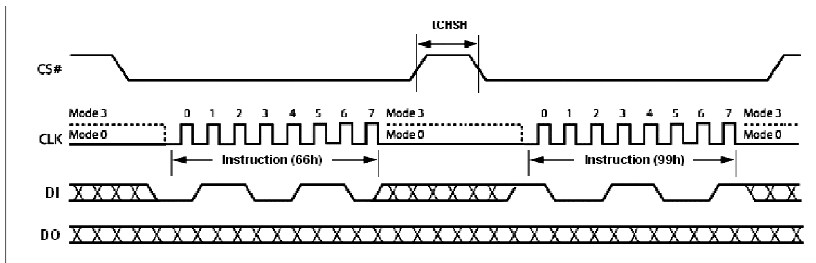
Reset-Enable and Reset Sequence Diagram
