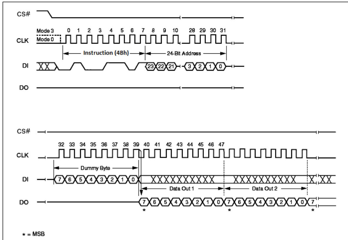
Read Unique ID Instruction Sequence Diagram
