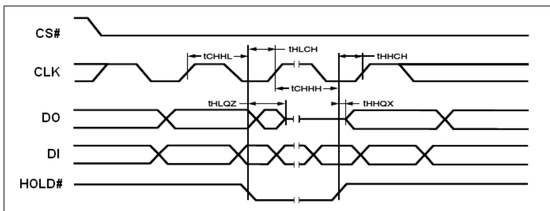
Hold Timing
