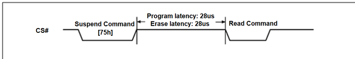
Suspend to Read Latency
