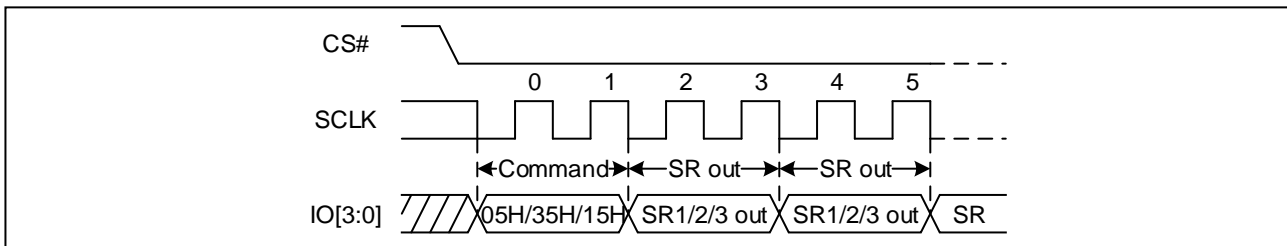
Figure 10. Read Status Register Sequence Diagram (QPI)
