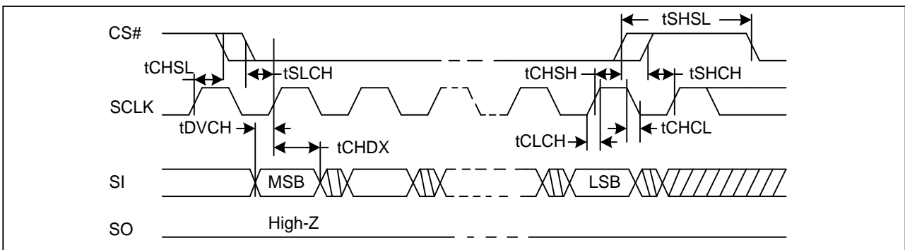
Figure 71. Input Timing
