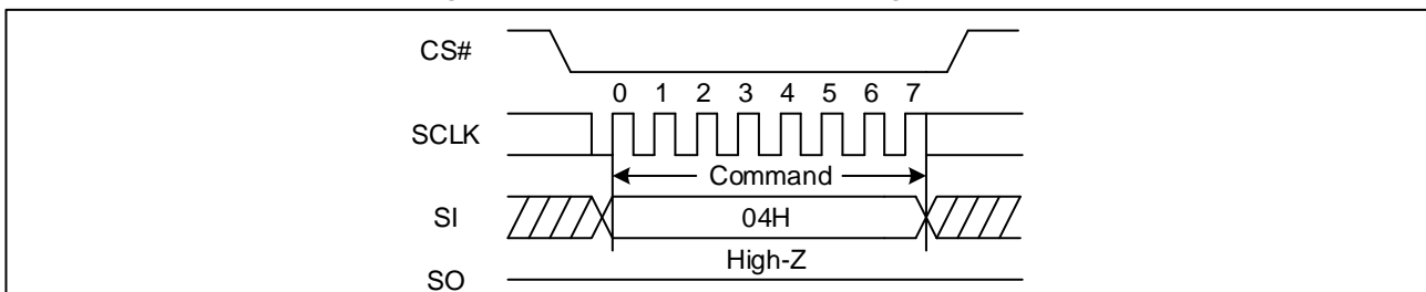
Figure 7. Write Disable Sequence Diagram (SPI)
