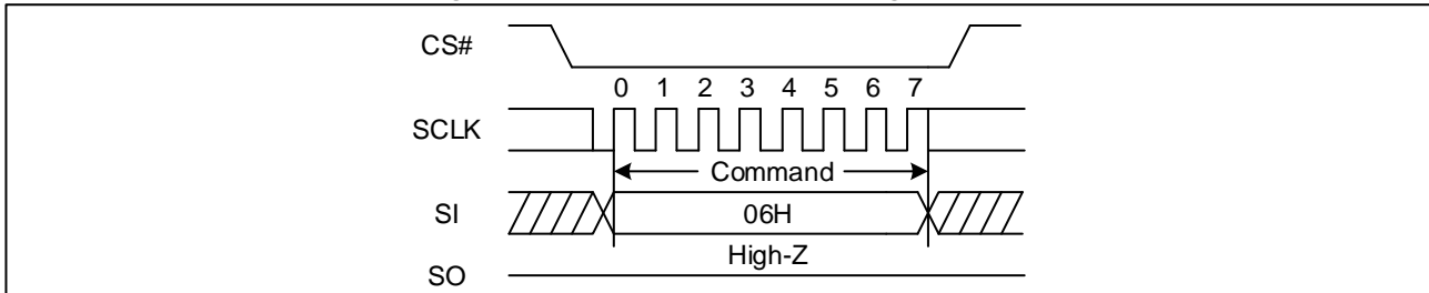
Figure 5. Write Enable Sequence Diagram (SPI)
