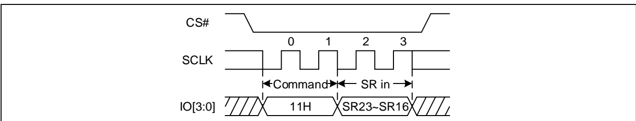
Figure 14. Write Status Register-3 Sequence Diagram (QPI)
