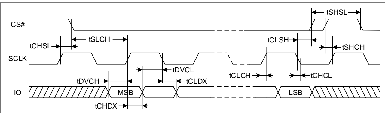
Figure 73. Serial Input Timing (DTR)
