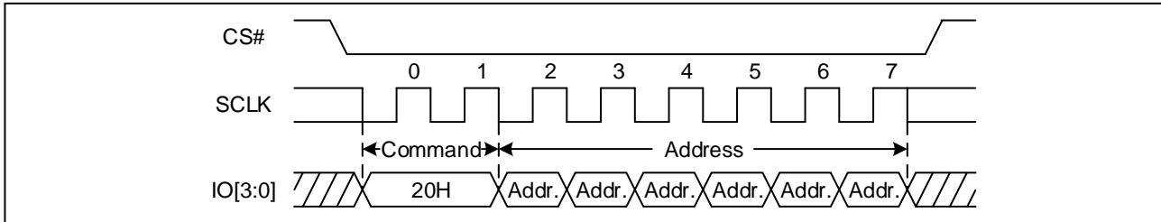
Figure 37. Sector Erase Sequence Diagram (QPI)
