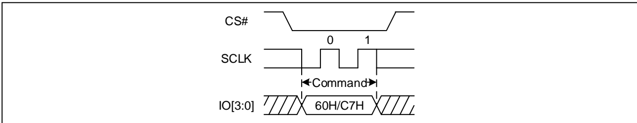
Figure 43. Chip Erase Sequence Diagram (QPI)
