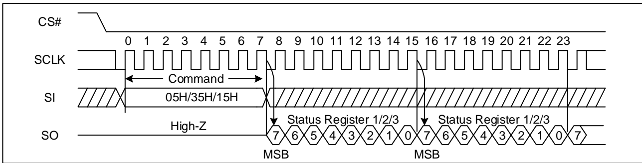
Figure 9. Read Status Register Sequence Diagram (SPI)
