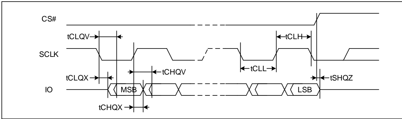
Figure 74. Serial Output Timing (DTR)
