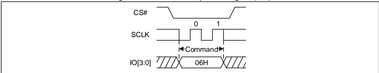
Figure 6. Write Enable Sequence Diagram (QPI)
