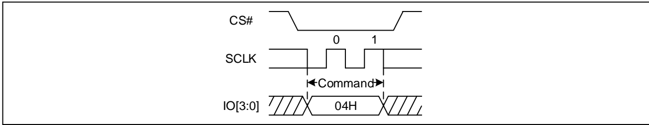
Figure 8. Write Disable Sequence Diagram (QPI)
