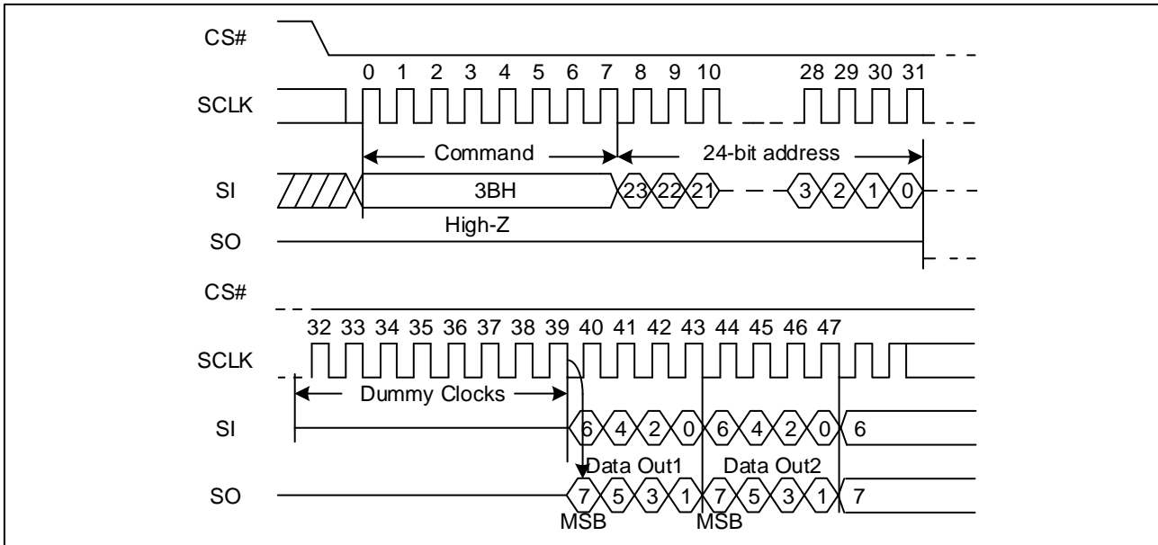
Figure 20. Dual Output Fast Read Sequence Diagram
