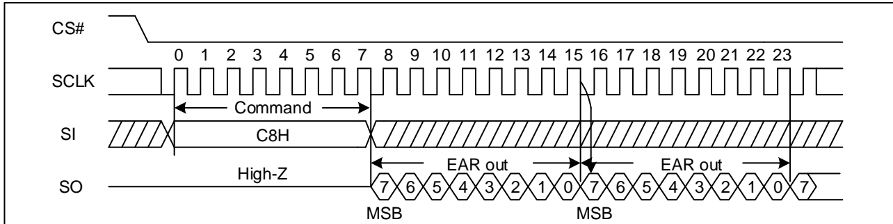
Figure 13 Read Extended Register Sequence Diagram (SPI)
