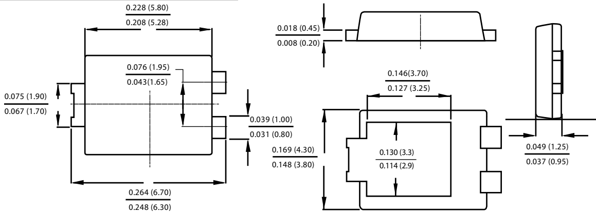
TO-277
