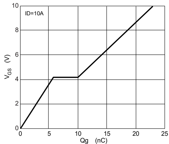
FIG. 5-Gate Charge Characteristics
