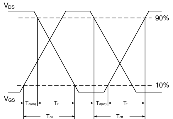
FIG. 6-Switching Time Waveform
