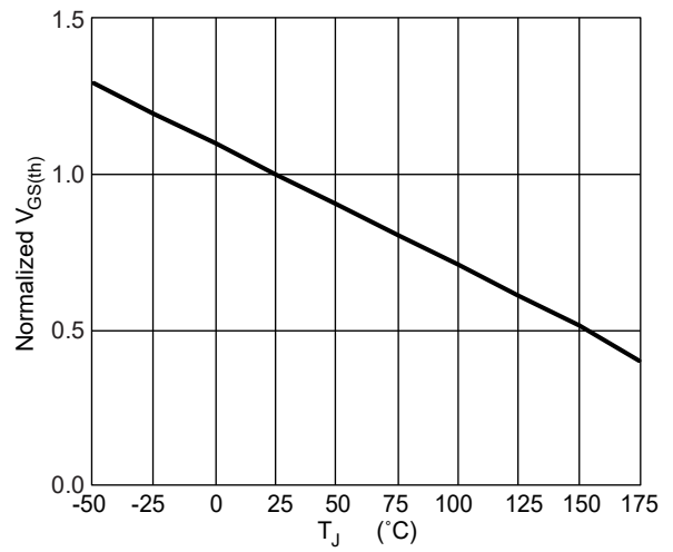
FIG. 4-Normalized V_{GS(th)} vs. T_J
