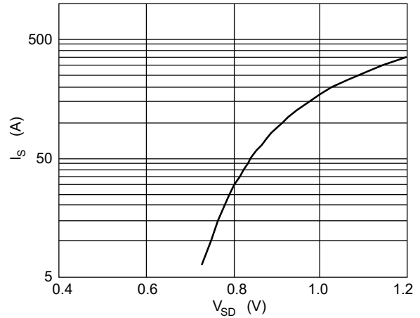
FIG. 2-Body-Diode Forward Characteristics
