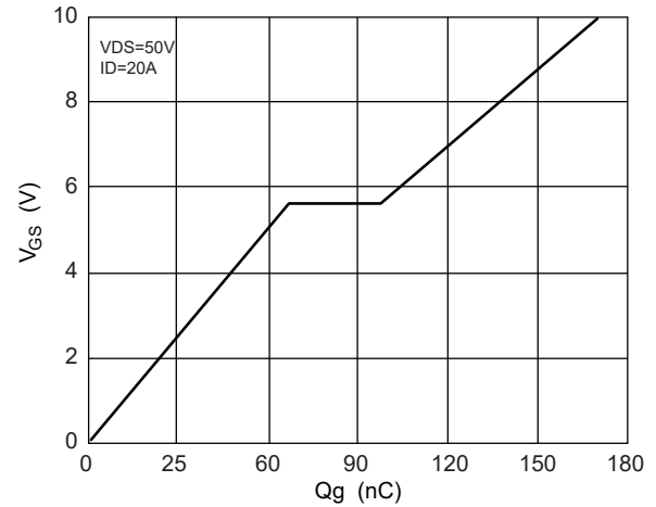
FIG. 4-Gate Charge Characteristics
