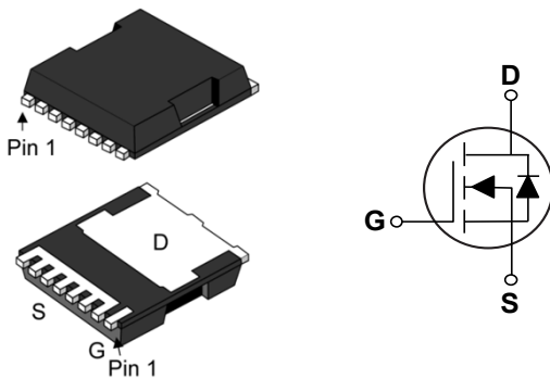
TOLLA-8 Pin Configuration
