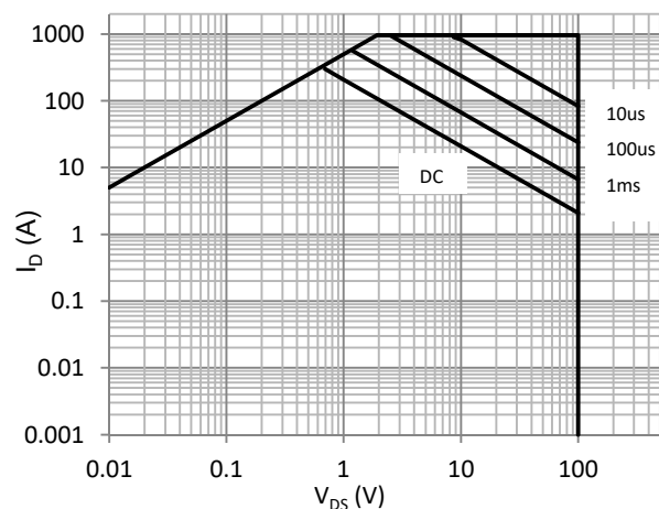
FIG. 5-Safe Operation Area
