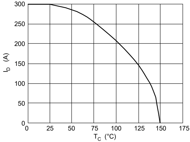
FIG. 1-Drain Current
