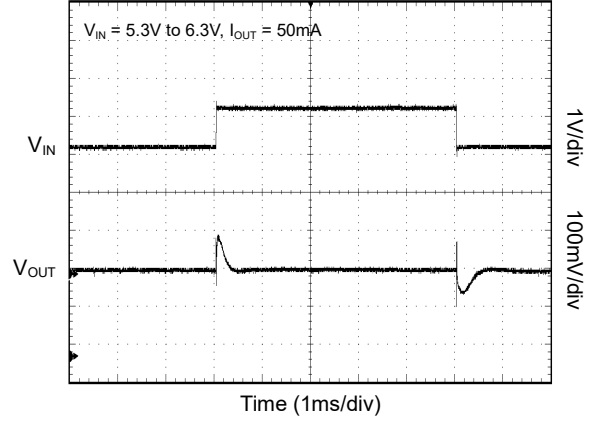
Line-Transient Response
