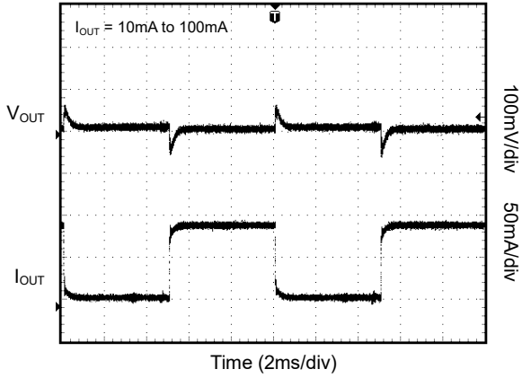
Load-Transient Response
